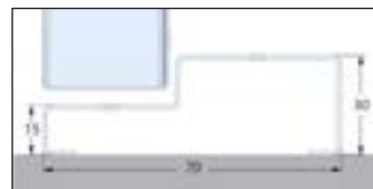
Standard 30mm open out rebated threshold (Optional on insulated doors, must be specified if required)
