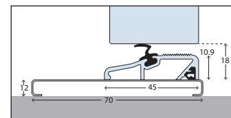
Standard inward opening threshold
