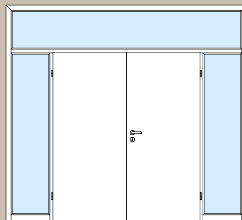
Double-leaf, 2 side elements, 1 transom light
